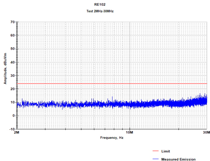
Plot 1. 4: RE102 test results within 30 – 200 MHz, vertical polarization
